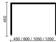
Melfi - 01G (Front view)
