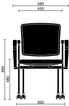
Flap 01W (Front view) Flap 01B (Front view)
