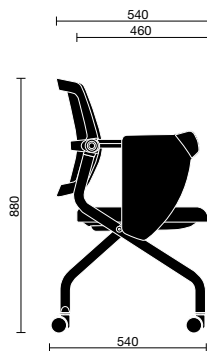
Flap 03W (Side view) Flap 03B (Side view)
