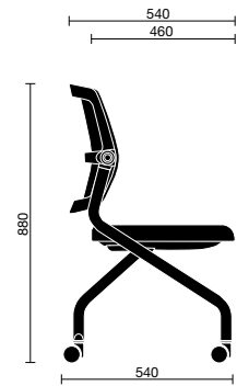
Flap 02W (Side view) Flap 02B (Side view)
