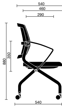
Flap 01W (Side view) Flap 01B (Side view)
