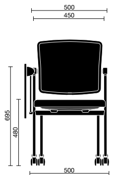
Flap 03W (Front view) Flap 03B (Front view)
